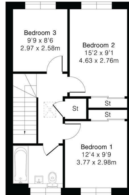
First Floor (Plot 04)
